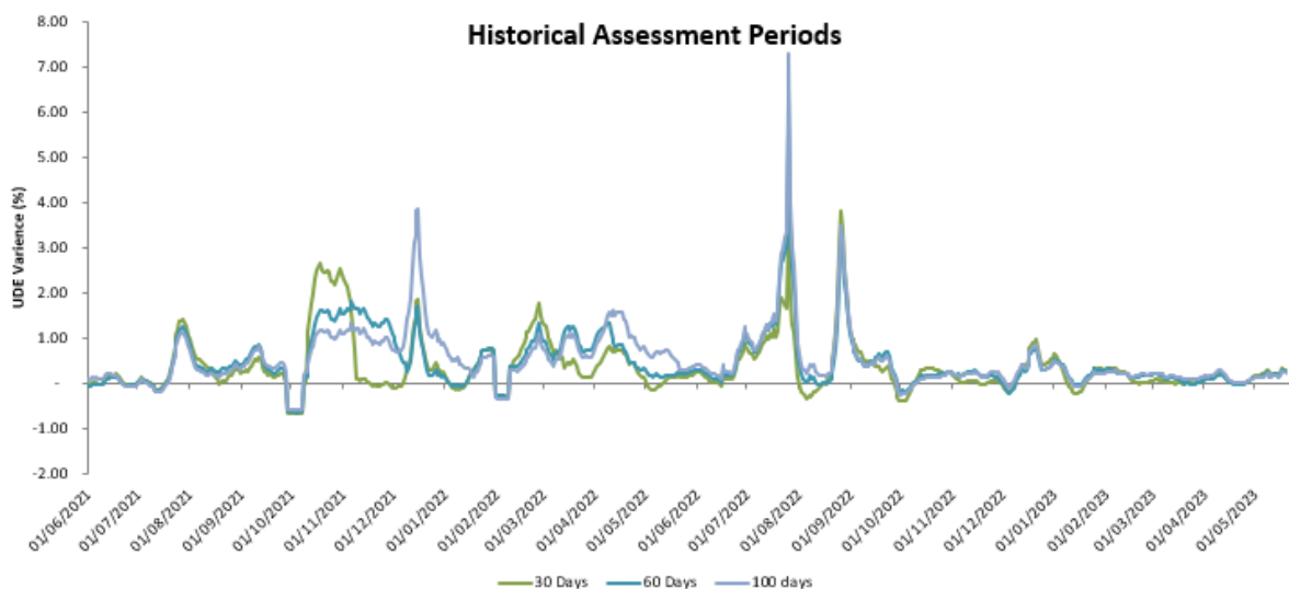
Figure 8: Effect of Different HAP on UDE Variance for Supplier with Steady Demand
