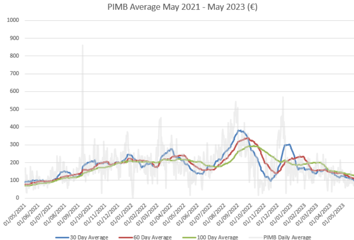
Figure 9: PIMB Average over 30, 60 and 100 days
