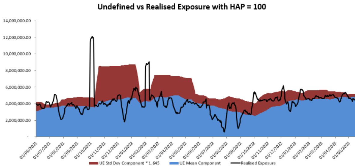
Figure 6: Estimated Undefined Exposure vs Realised Undefined Exposure with DINHAP = 100
