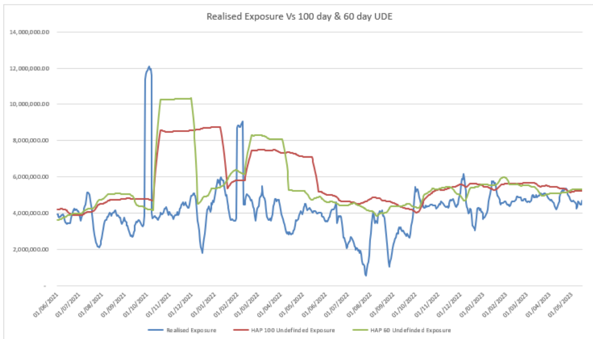
Figure 7: Realised Undefined Exposure compared to estimated Undefined Exposure DINHAP of 100 and 60 days
